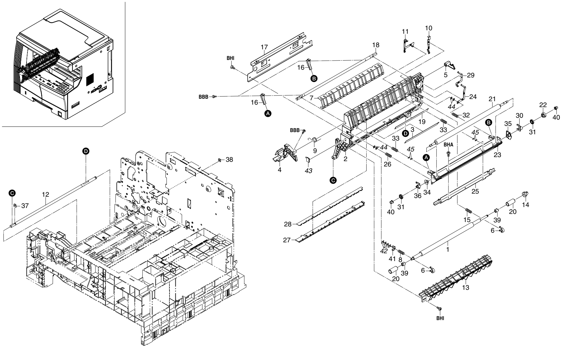
FIG. 4 CONVEYING SECTION
